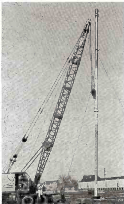
RCA's traveling wave antenna for vhf. Page 112
